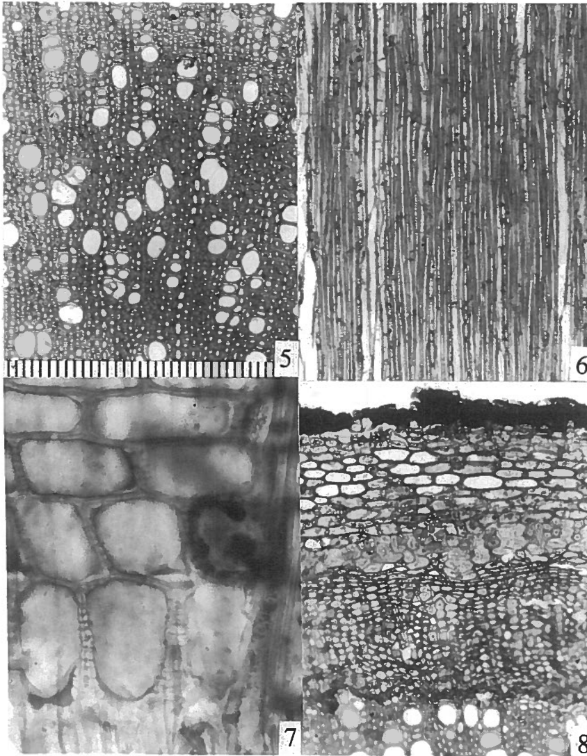
Figs. 5-8. Phaulothamnus spinescens , sections of wood (5-7) and bark (8). Fig. 5. Transsection; vessels are mostly grouped. Fig. 6. Tangential section; rays inconspicuous, composed mostly of upright cells. Fig. 7. Radial section, procumbent ray cells at top, upright cells at bottom. Fig. 8. Transsection, phellem at top, secondary xylem at bottom; outer cortex consists of oval parenchyma cells, inner cortex is comprised of pale gray fibers. Figs. 5, 6, 8, scale below Fig. 5 (divisions = 10 \mu m); Fig. 7, scale below Fig. 3.
