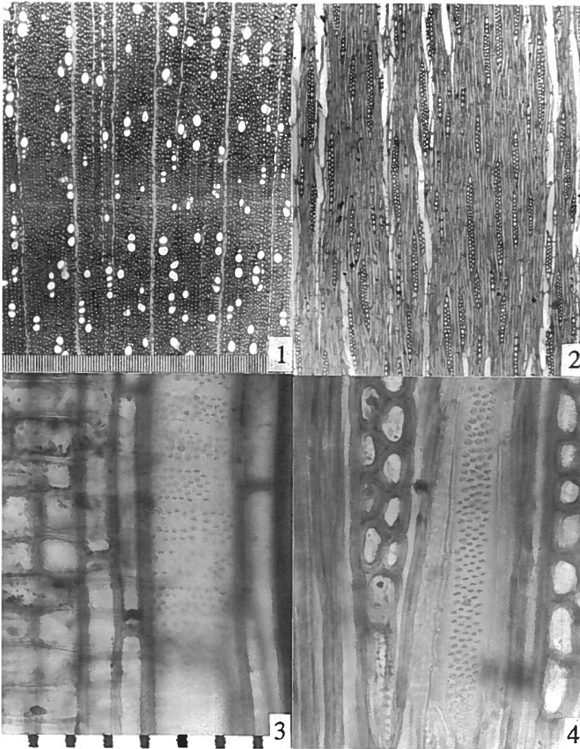
Figs. 1–4. Achatocarpus praecox , wood sections. Fig. 1. Transverse section; vessels in center are slightly narrower, indicating inconspicuous growth ring. Fig. 2. Tangential section; rays are biseriate or uniseriate. Fig. 3. Radial section; an axial parenchyma strand touches the left side and another the right side of the vessel. Fig. 4. Tangential section; tip of biseriate ray, left; alternate minute pits on vessel. Figs. 1–2, scale below Fig. 1 (divisions = 10 \mu\text{m} ); Figs. 3–4, scale below Fig. 3 (divisions = 10 \mu\text{m} ).
